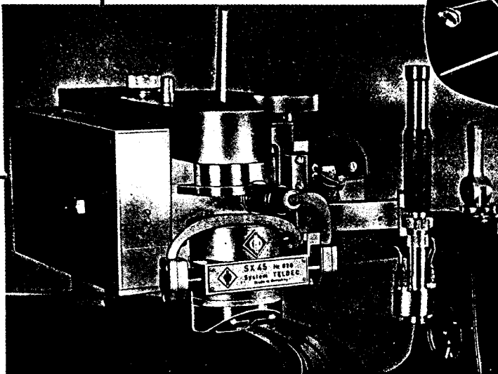
SX-45 mounted on Automatic Cutterhead Suspension of AM-32B Master Disk Recording Lathe.
