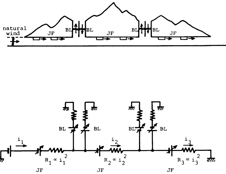
Fig. 3 Analogy of ventilation characteristics to electrical circuit
